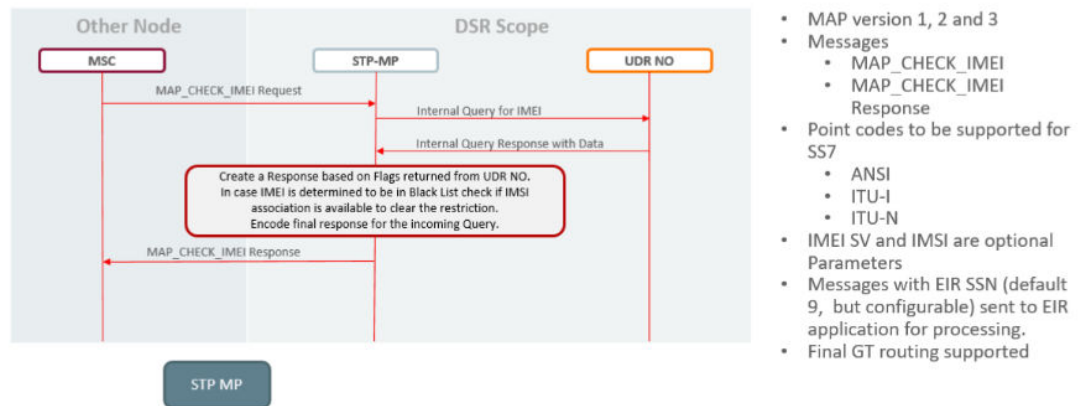
Figure 2-75 SS7 EIR call flow
