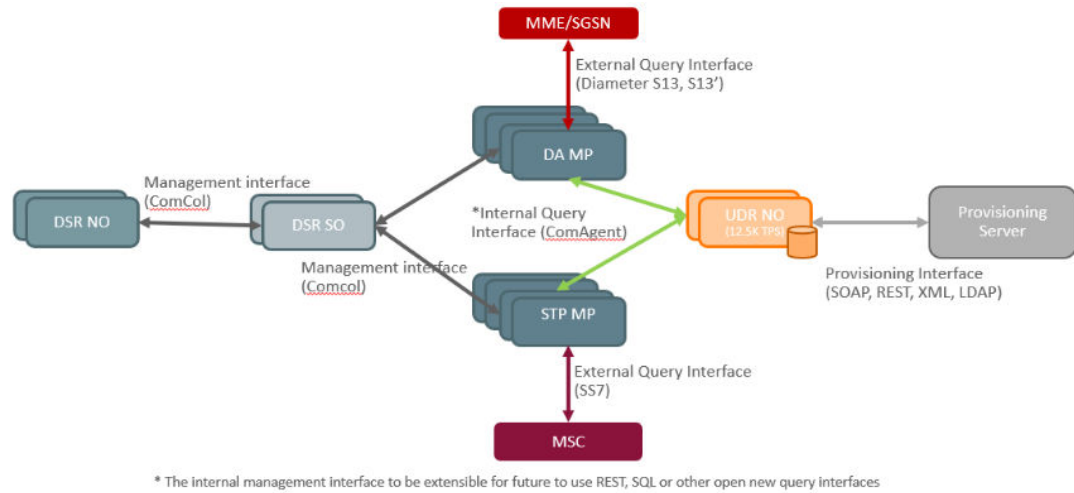
Figure 2-74 EIR solution architecture.
